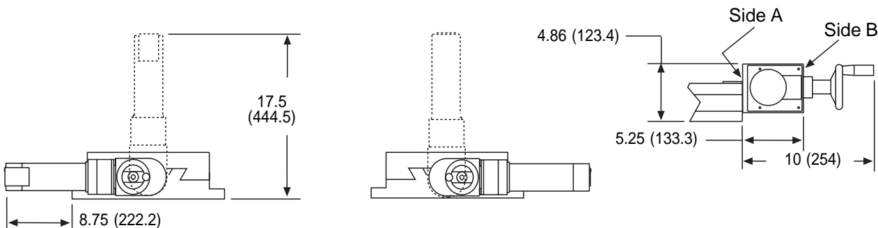
Side A mounted to bed (multiple feed positions shown)
